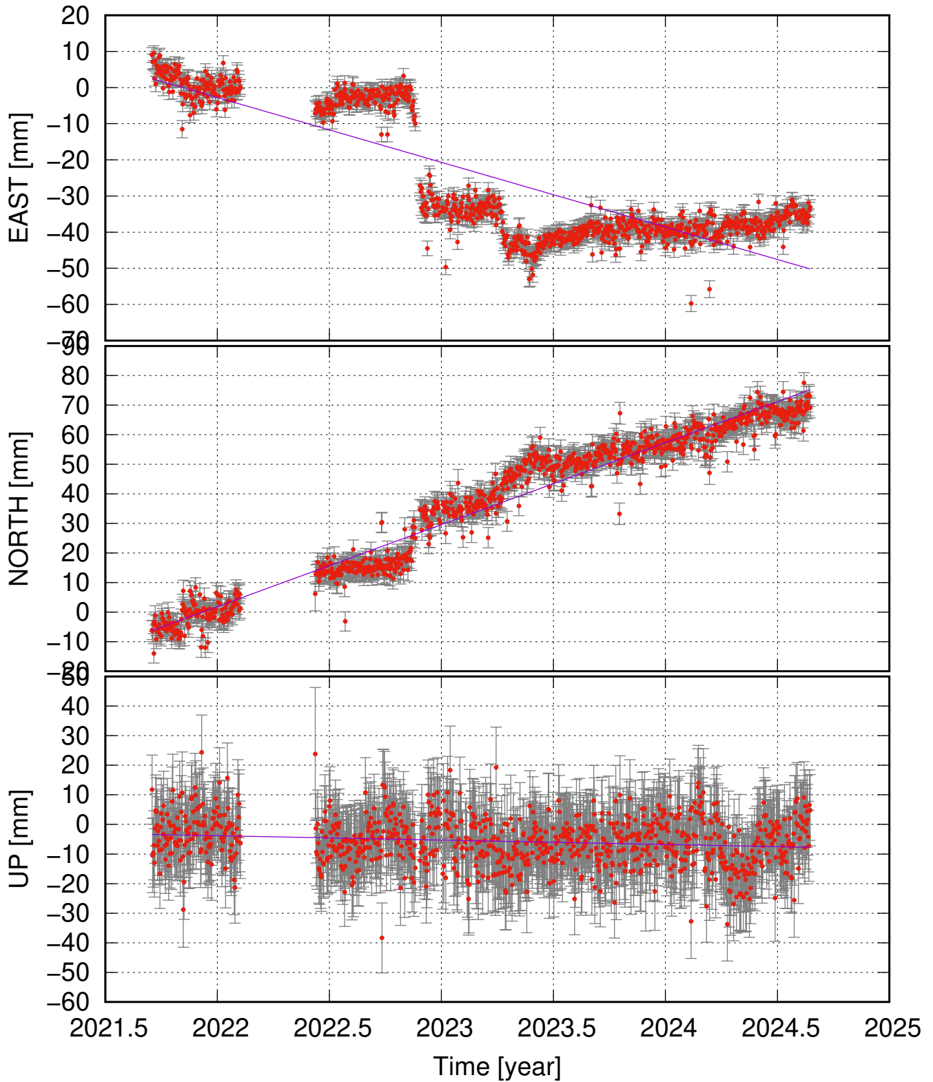
SEY6 (65.26, -13.99) time series (ITRF 2014) ve = -17.93 \pm 3.36 ; vn = 27.72 \pm 1.77 ; vu = -1.48 \pm 2.73 mm/yr
