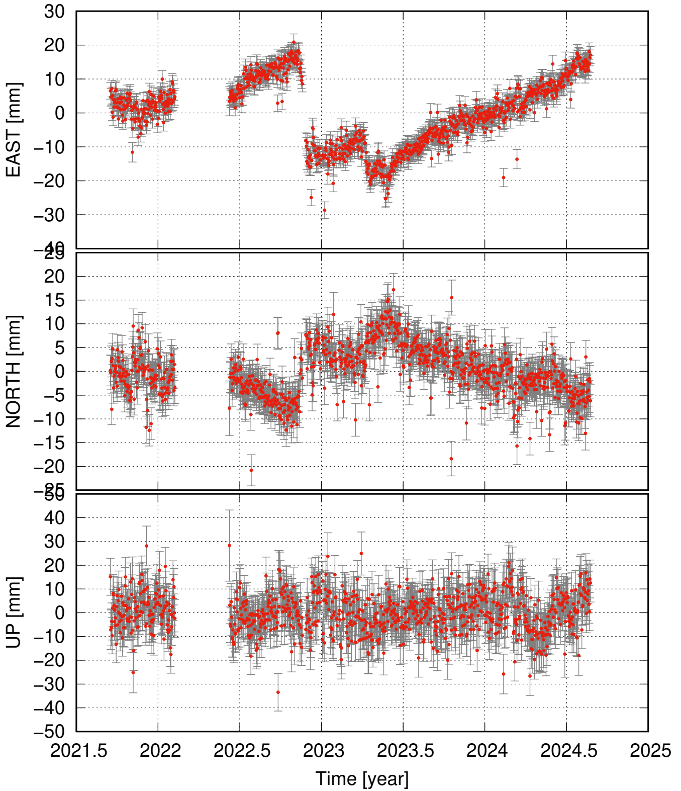
SEY6 residual time series
