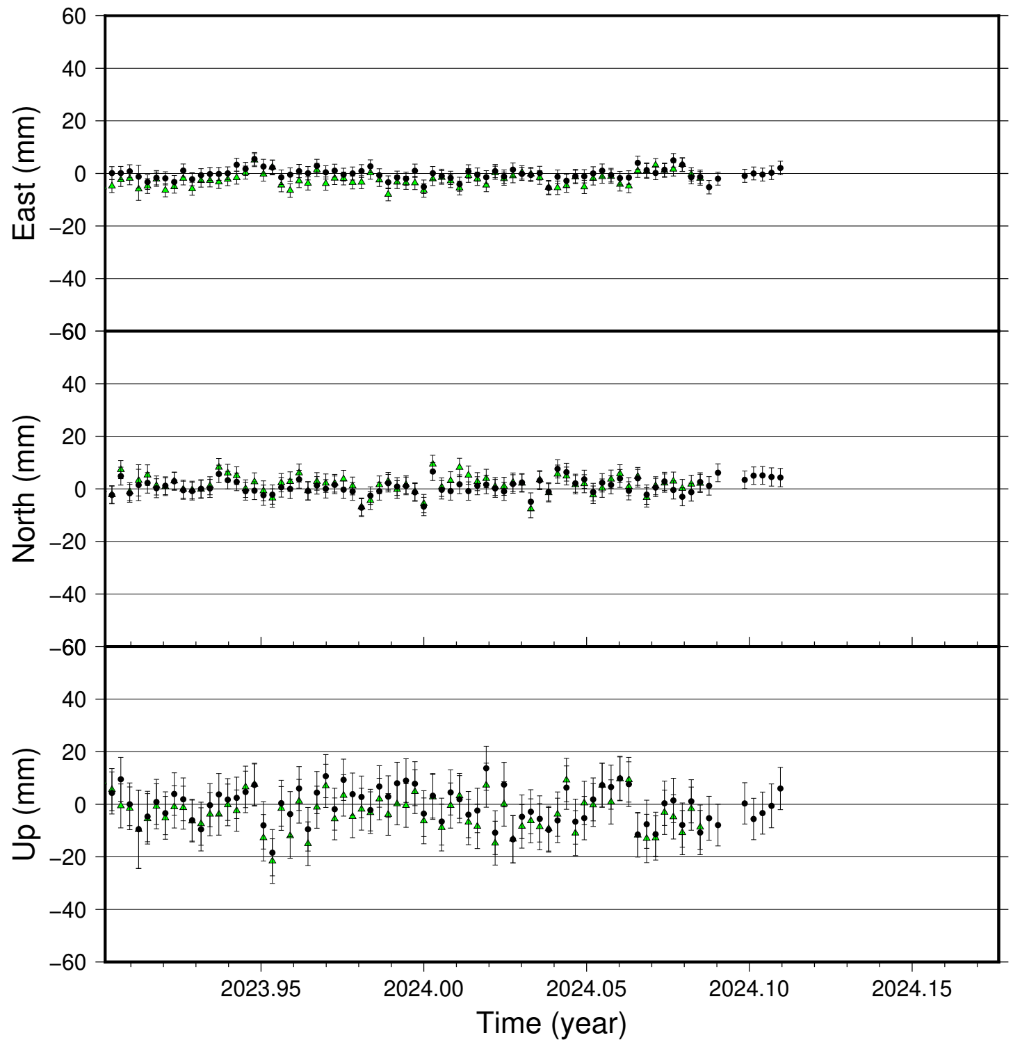
SEY6 time series (IGS 2014), last 100 days
