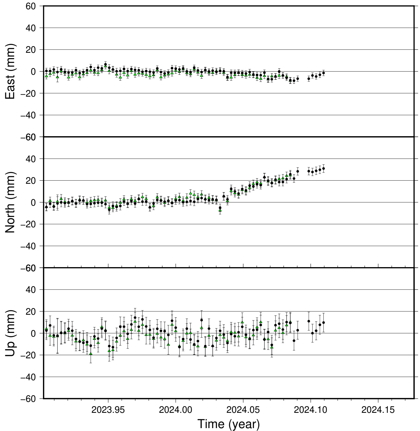
SEY5 time series (IGS 2014), last 100 days
