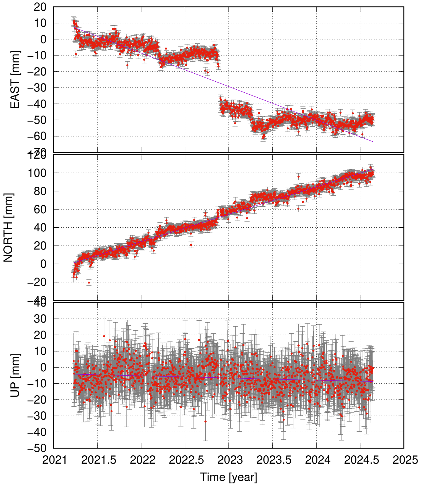
SEY4 (65.26, -14.00) time series (ITRF 2014) v_e = -20.69 \pm 2.67 ; v_n = 30.14 \pm 1.35 ; v_u = -1.34 \pm 2.31 mm/yr
