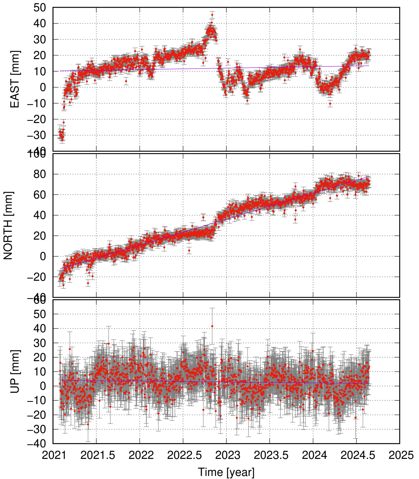
SEY3 (65.26, -13.99) time series (ITRF 2014) v_e = 0.90 \pm 2.69 ; v_n = 25.29 \pm 1.38 ; v_u = -0.60 \pm 2.36 mm/yr
