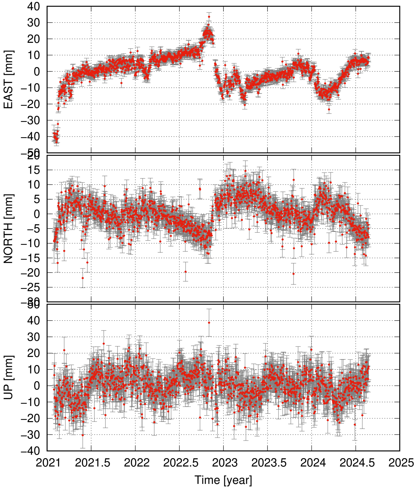
SEY3 residual time series (some major events removed as well)
