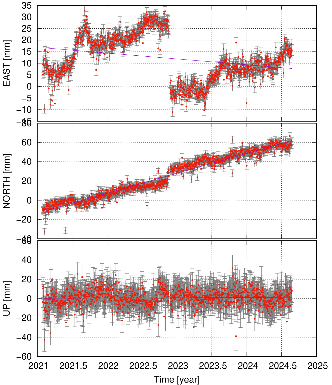
SEY2 (65.26, -14.00) time series (ITRF 2014) v_e = -2.51 \pm 2.60 ; v_n = 20.66 \pm 1.30 ; v_u = 0.29 \pm 2.29 mm/yr
