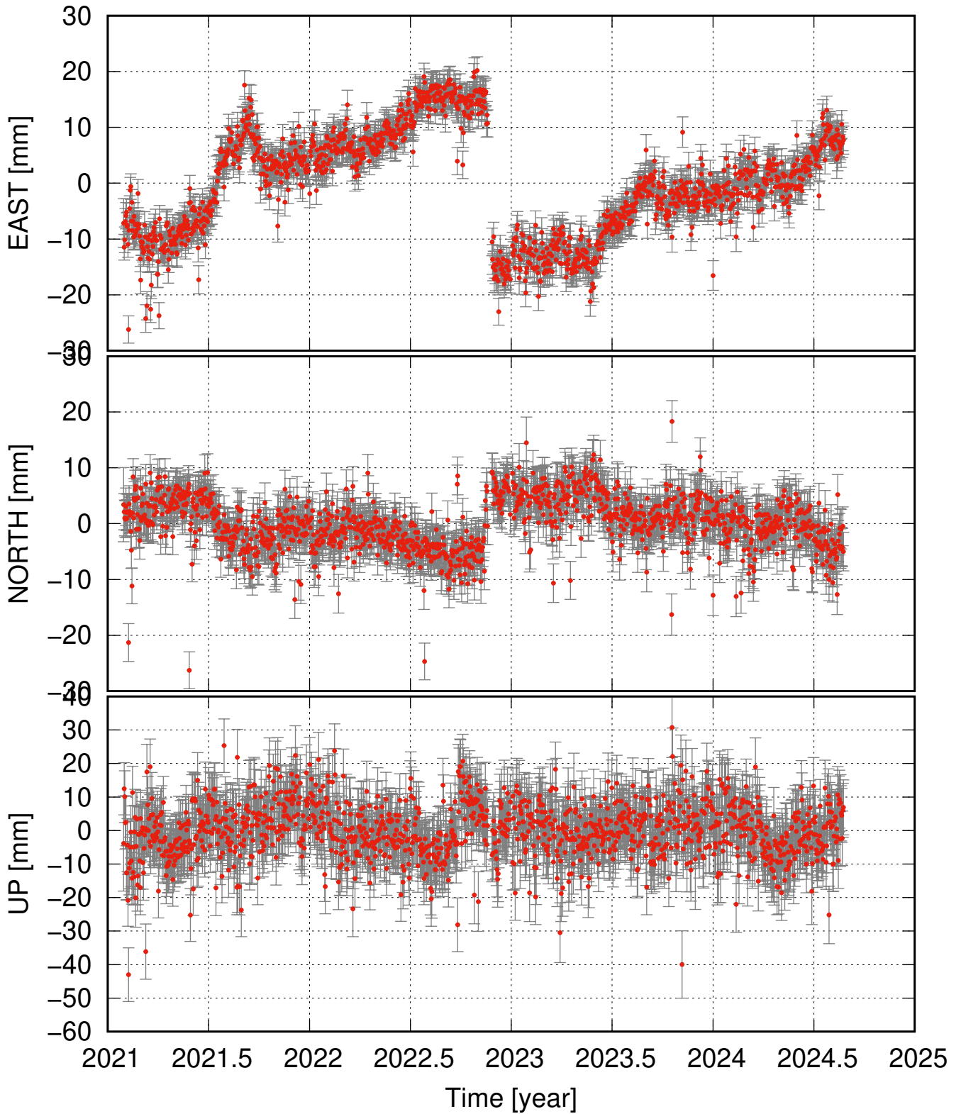
SEY2 residual time series (some major events removed as well)
