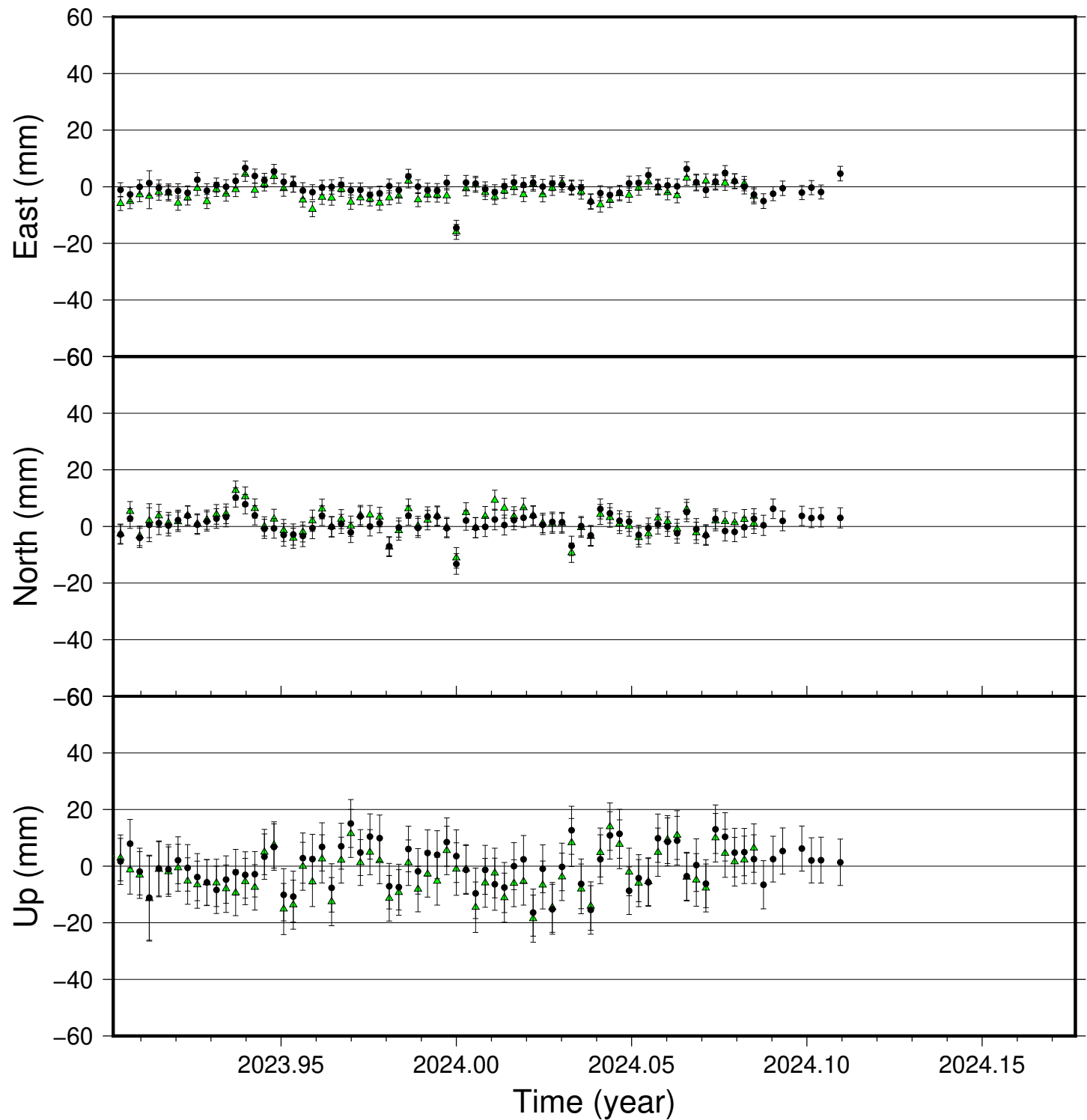
SEY2 time series (IGS 2014), last 100 days
