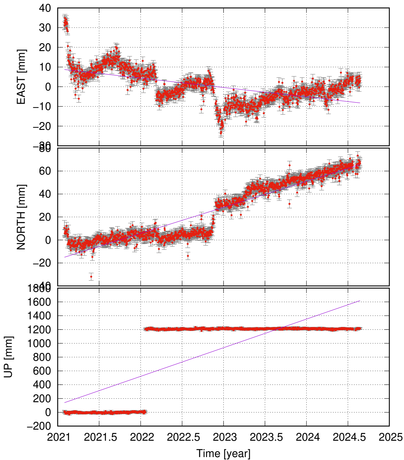
SEY1 (65.26, -13.99) time series (ITRF 2014) v_e = -4.77 \pm 1.87 ; v_n = 22.62 \pm 2.29 ; v_u = 414.98 \pm 96.08 mm/yr
