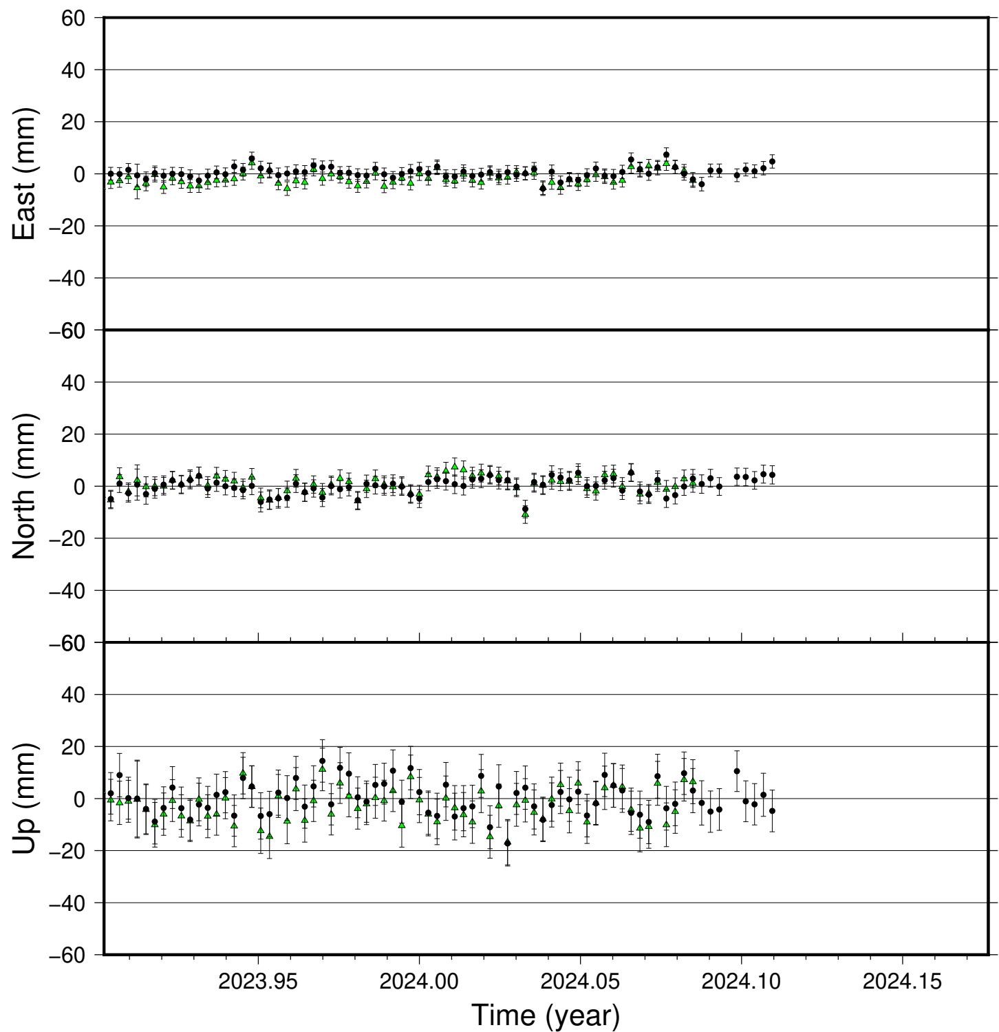
SEY1 time series (IGS 2014), last 100 days
