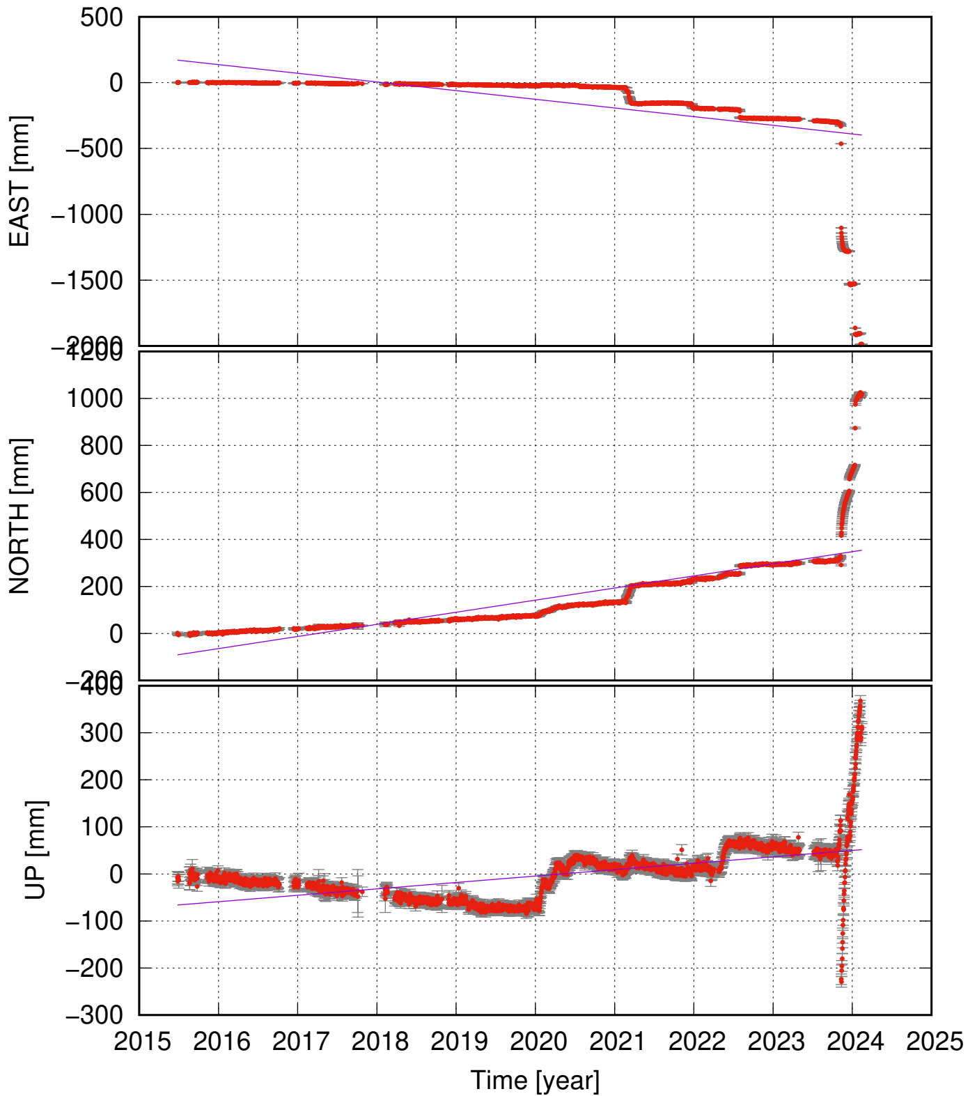
SENG (63.88, -22.43) time series (ITRF 2014) ve = -65.75 ± 28.14; vn = 51.56 ± 10.49; vu = 13.63 ± 5.42 mm/yr
