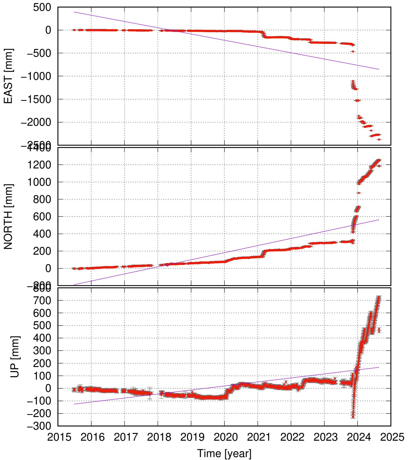
SENG (63.88, -22.43) time series (ITRF 2014) v_e = -135.97 \pm 50.33 ; v_n = 82.19 \pm 21.41 ; v_u = 31.96 \pm 12.50 mm/yr
