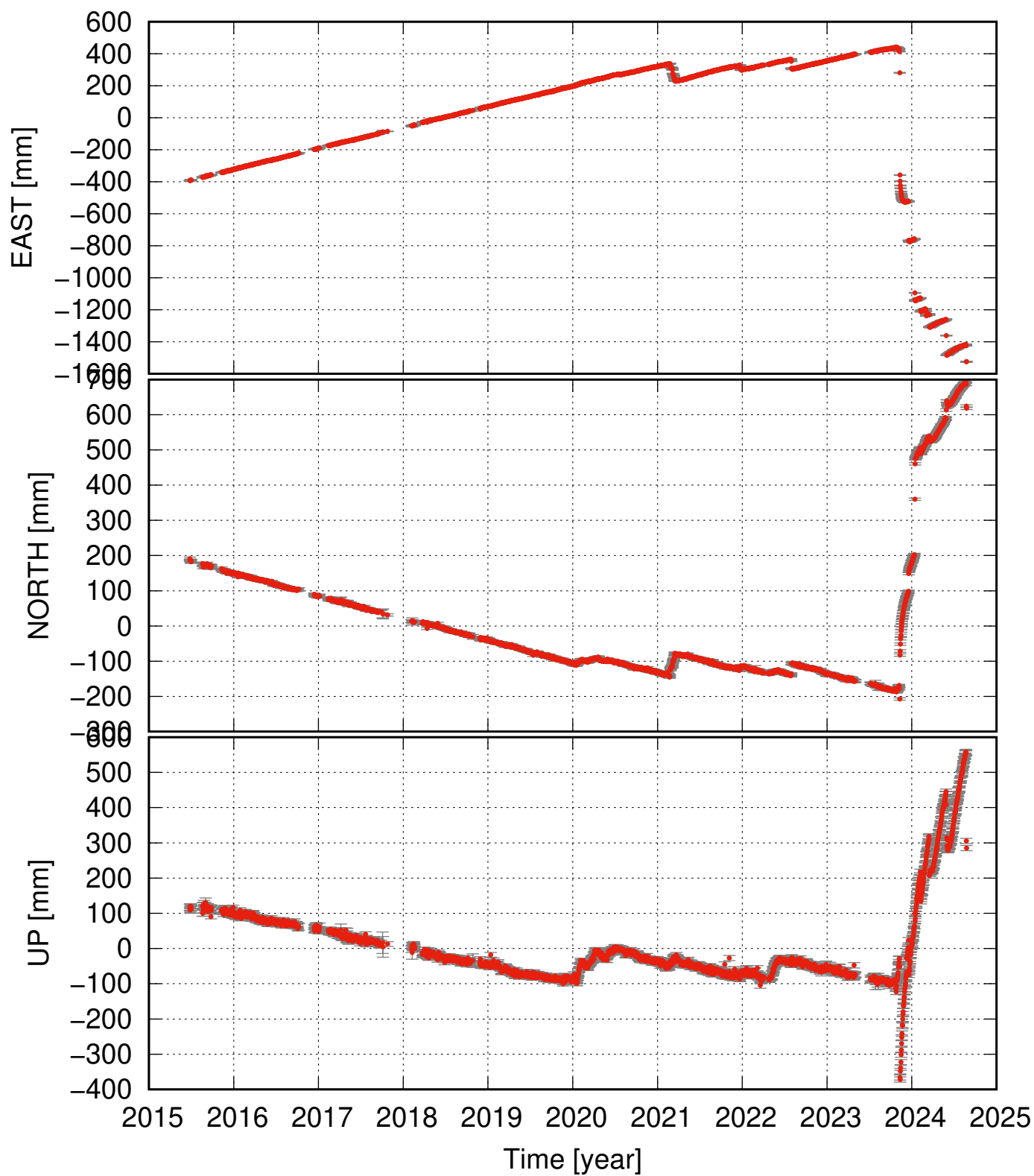
SENG residual time series
