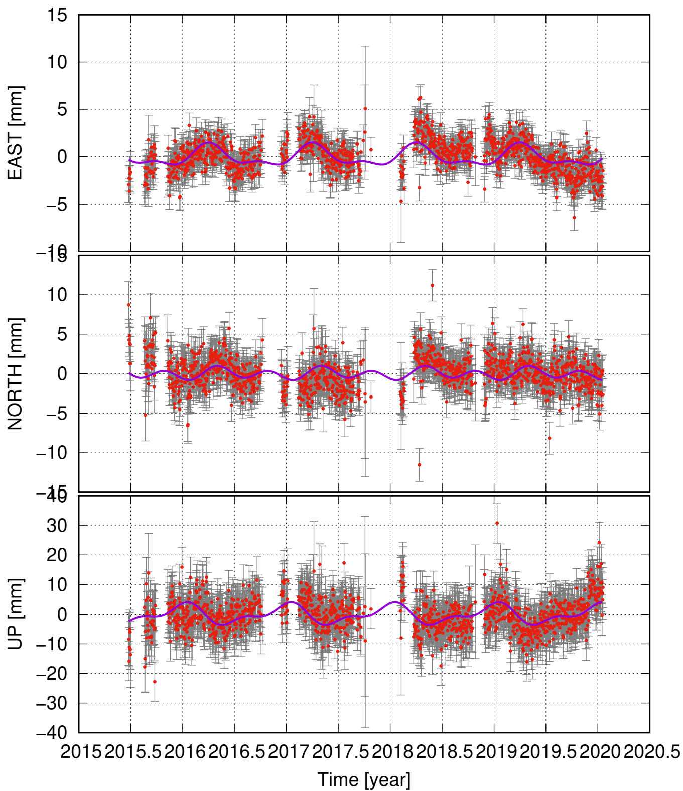
SENG seasonal fit
