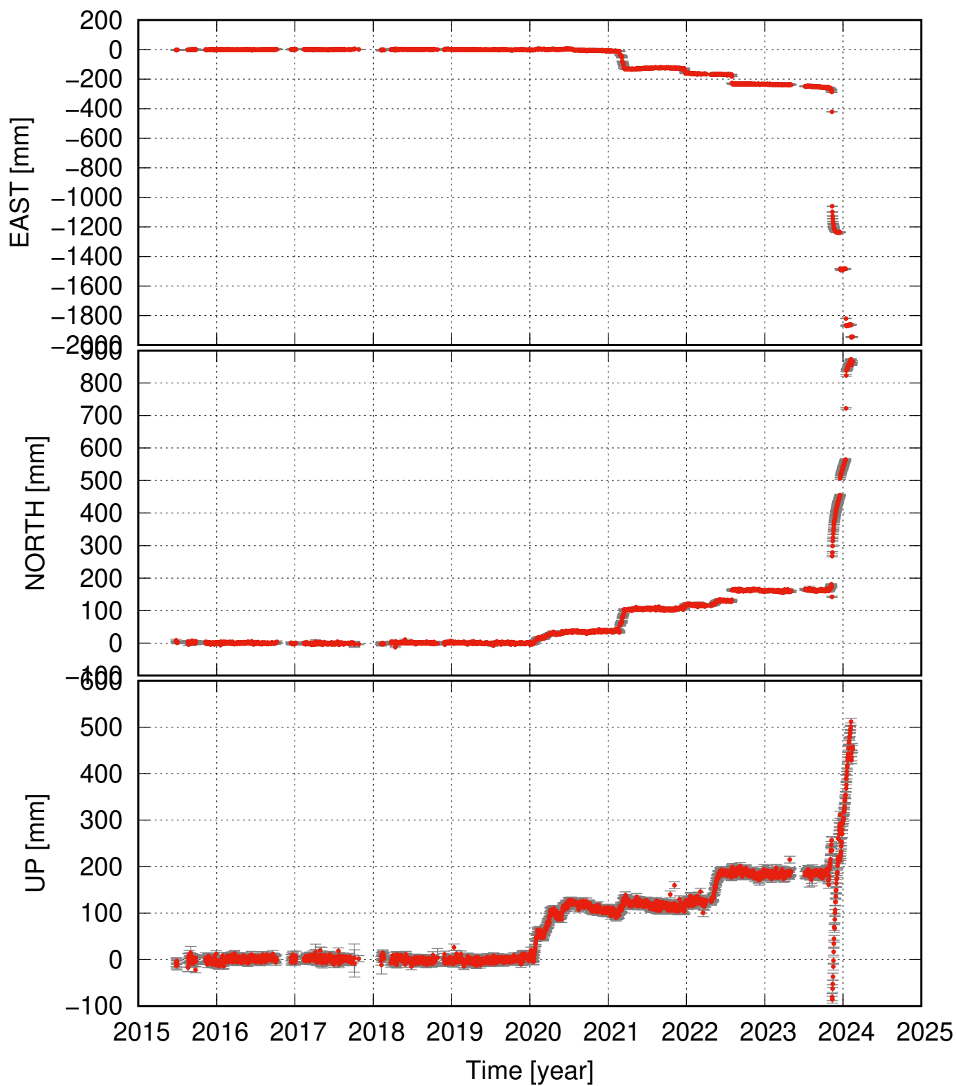
SENG detrended and seasonal signal removed
