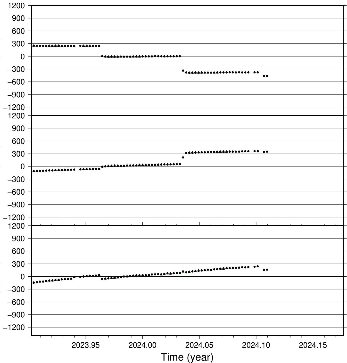
SENG time series (IGS 2014), last 100 days
