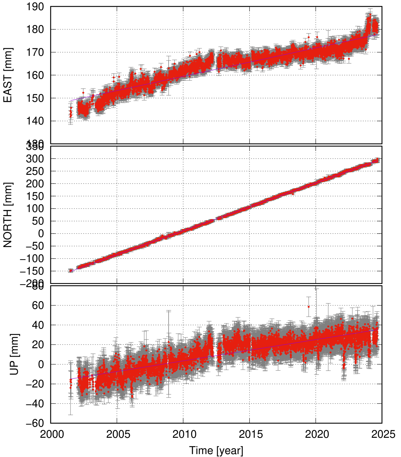
SELF (63.93, -21.03) time series (ITRF 2014) v_e = 1.24 \pm 0.11 ; v_n = 19.13 \pm 0.10 ; v_u = 2.17 \pm 0.31 mm/yr
