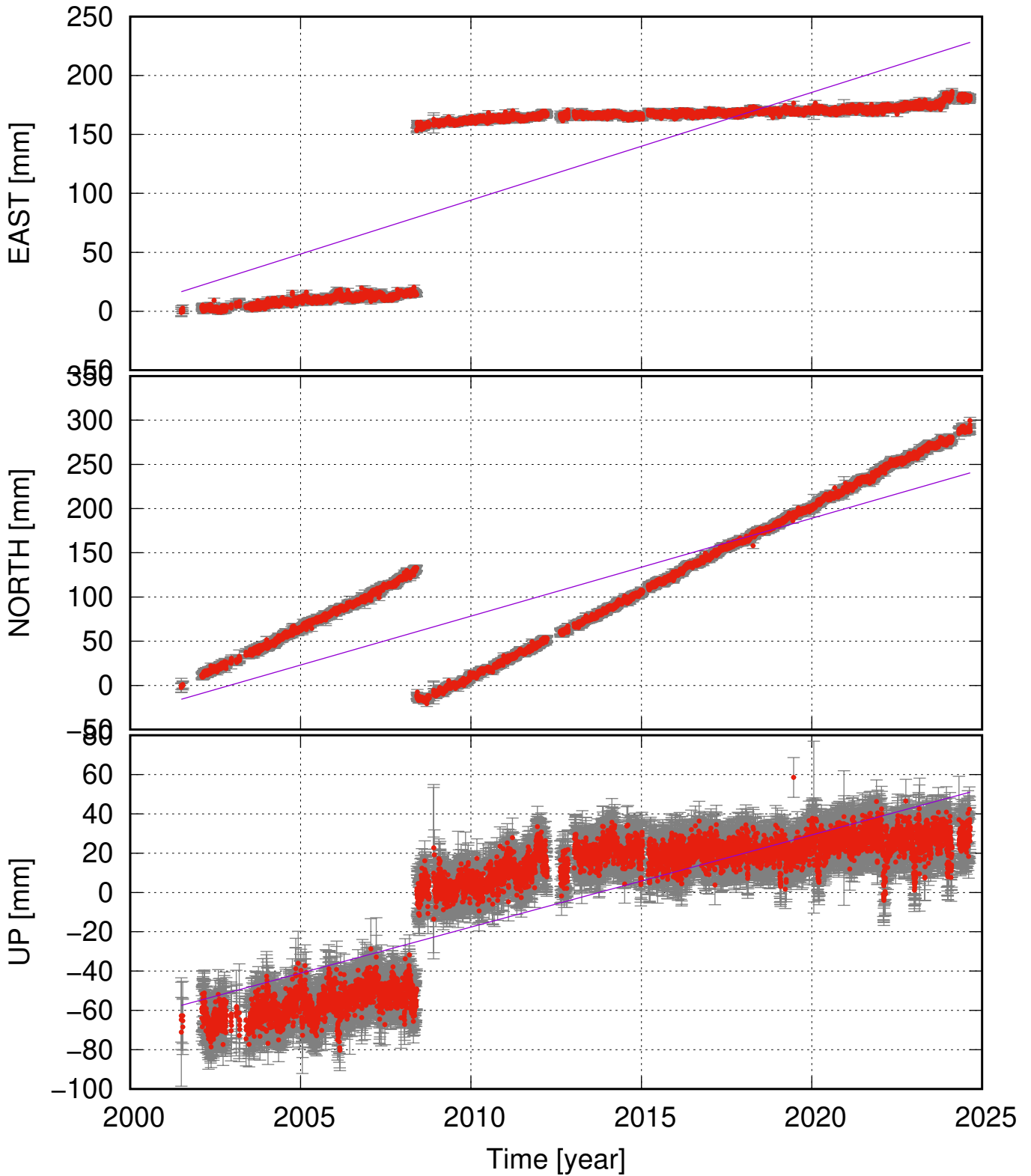
SELF (63.93, -21.03) time series (ITRF 2014) v_e = 9.14 \pm 1.79 ; v_n = 11.06 \pm 1.83 ; v_u = 4.69 \pm 0.75 mm/yr
