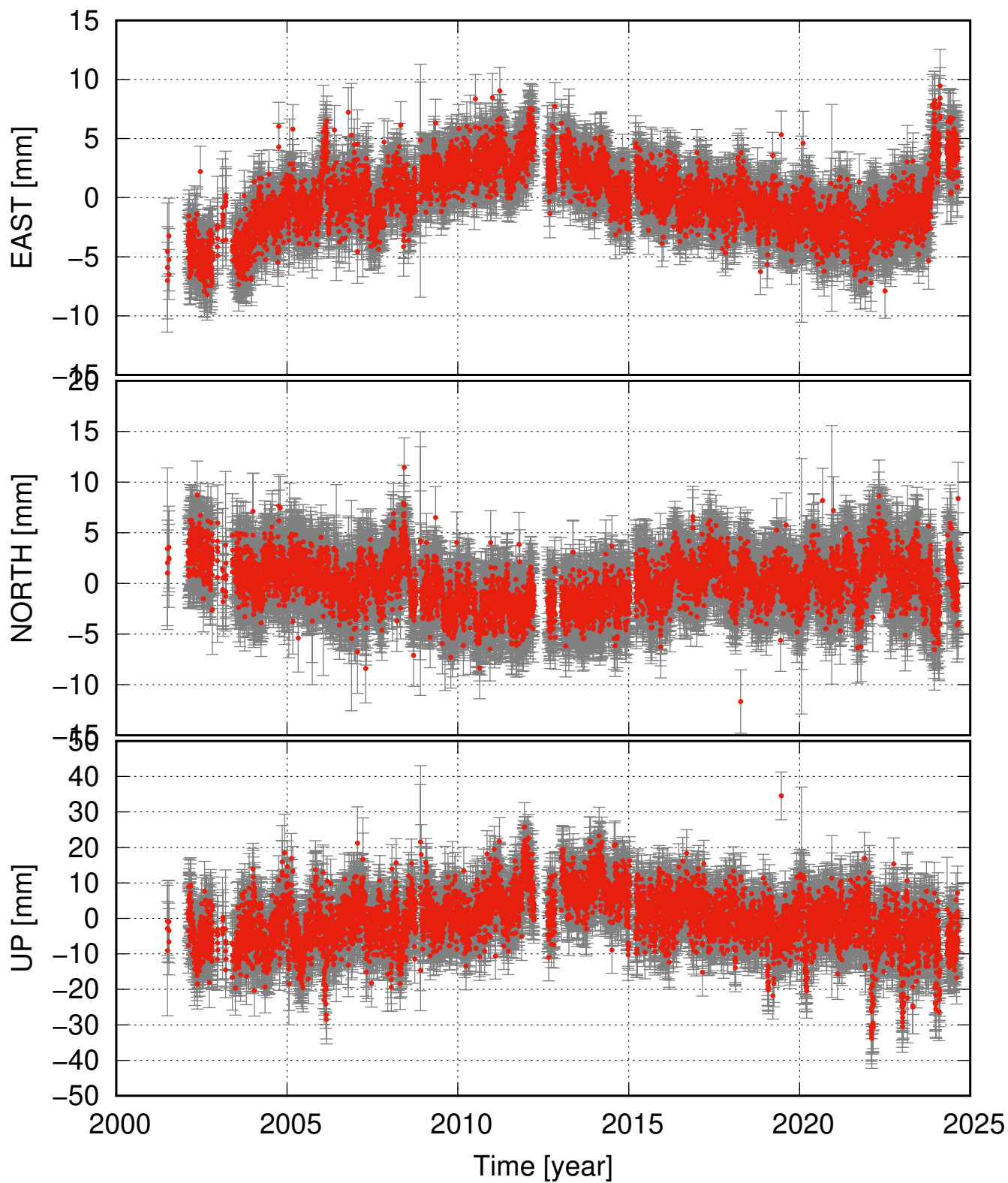
SELF residual time series (some major events removed as well)
