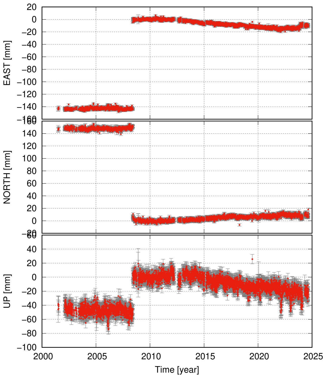
SELF detrended and seasonal signal removed
