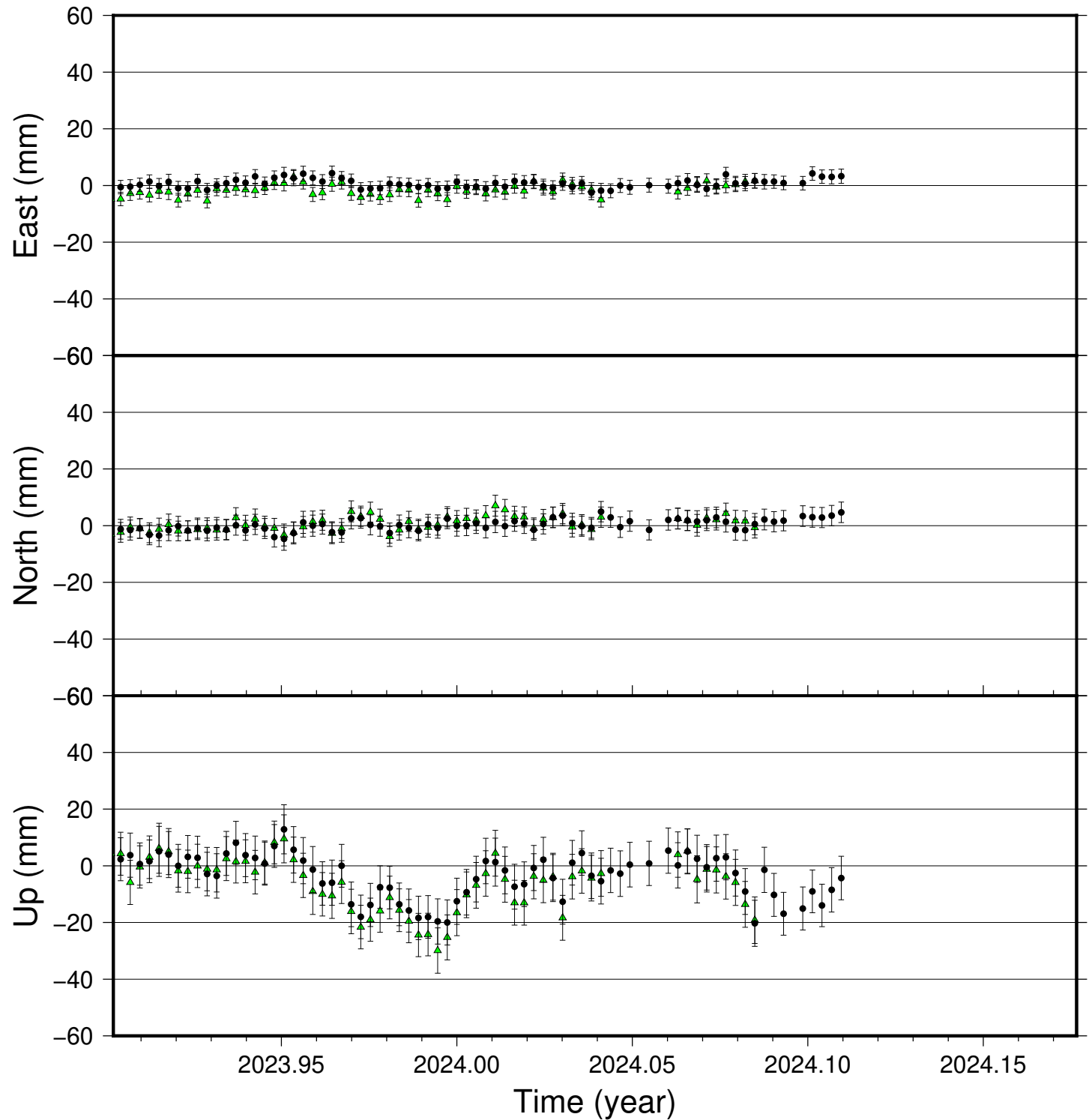
SELF time series (IGS 2014), last 100 days
