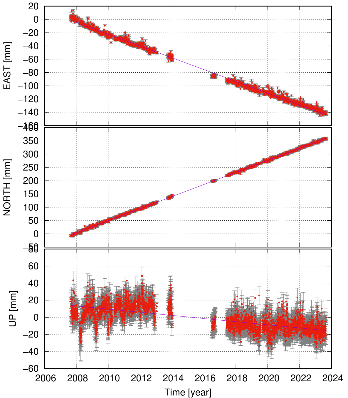
SAVI (65.99, -17.38) time series (ITRF 2014) v_e = -8.88 \pm 0.17 ; v_n = 22.71 \pm 0.14 ; v_u = -1.84 \pm 0.59 mm/yr
