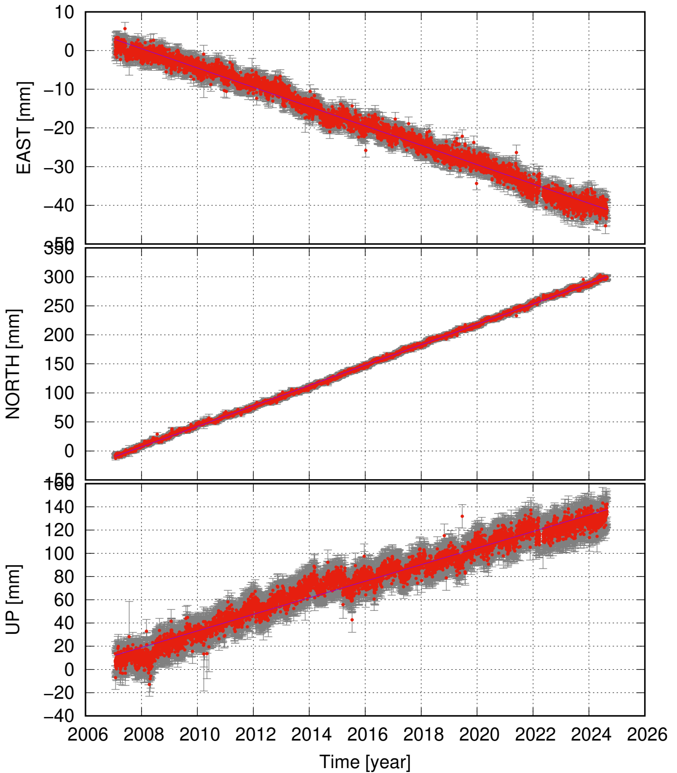
SAUR (63.98, -20.43) time series (ITRF 2014) v_e = -2.50 \pm 0.08 ; v_n = 17.59 \pm 0.13 ; v_u = 7.13 \pm 0.38 mm/yr
