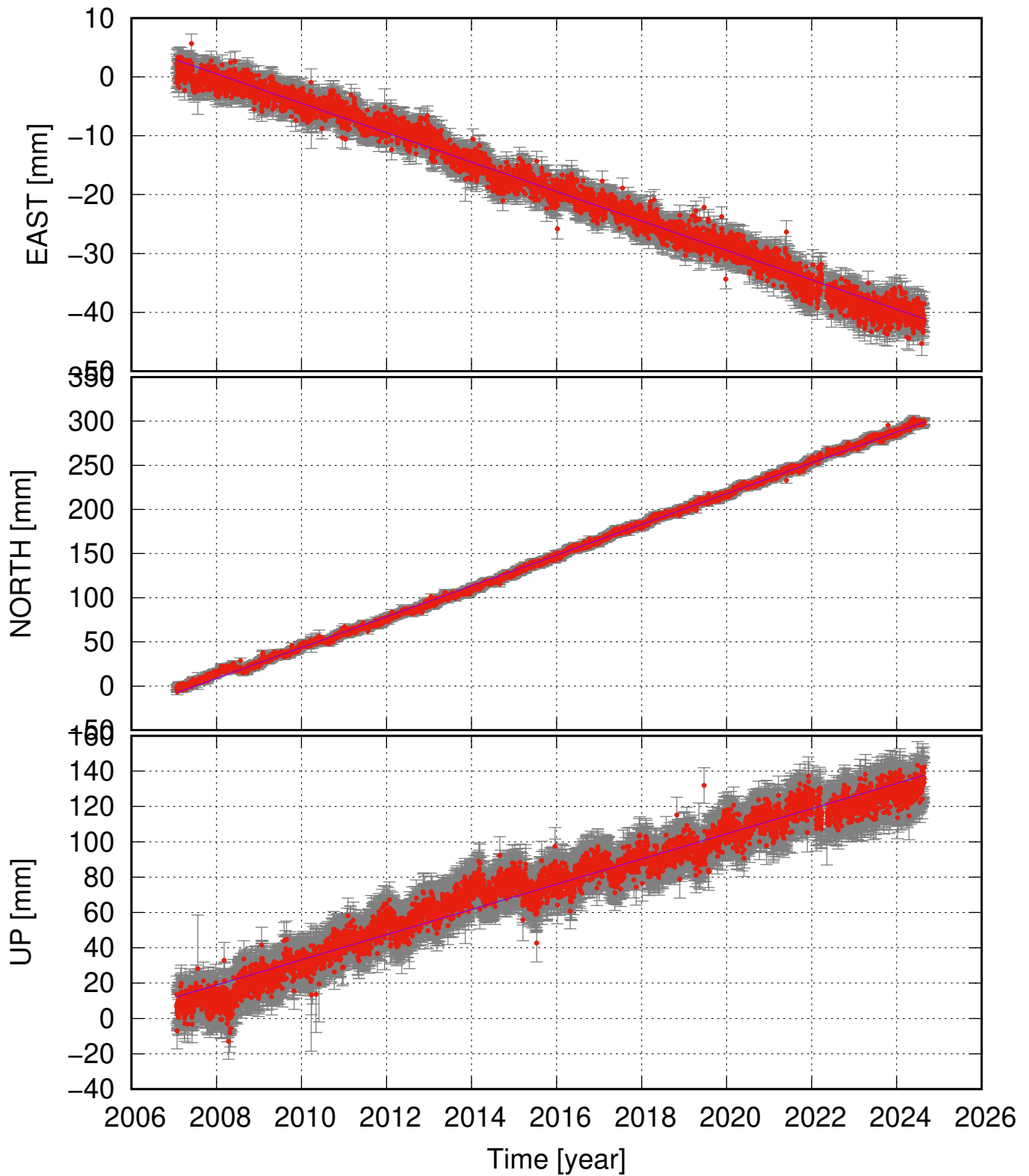
SAUR (63.98, -20.43) time series (ITRF 2014) v_e = -2.50 \pm 0.08 ; v_n = 17.43 \pm 0.17 ; v_u = 7.13 \pm 0.38 mm/yr
