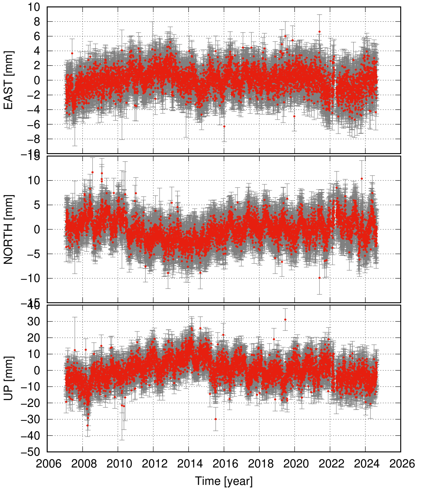
SAUR residual time series (some major events removed as well)
