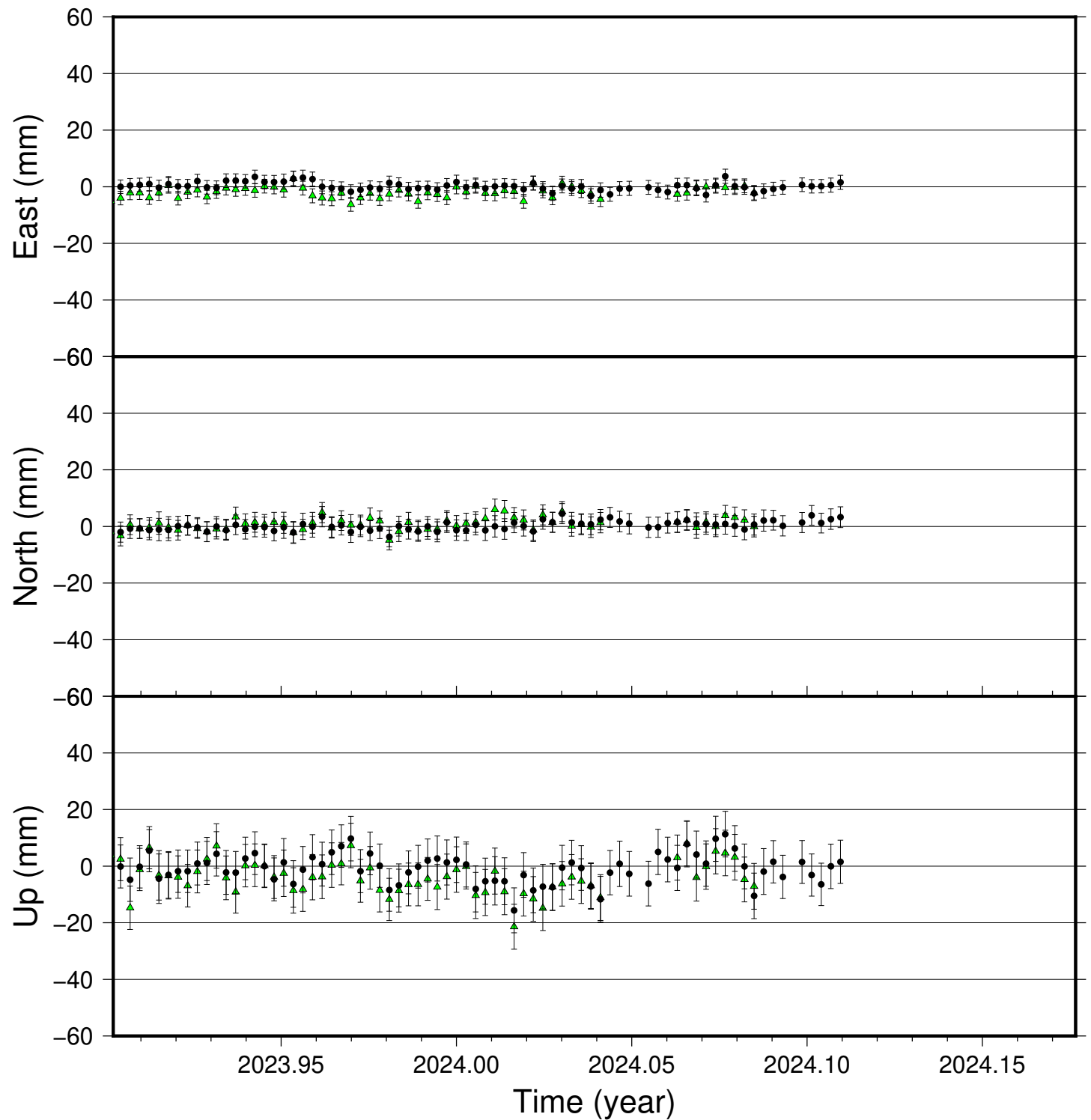
SAUR time series (IGS 2014), last 100 days
