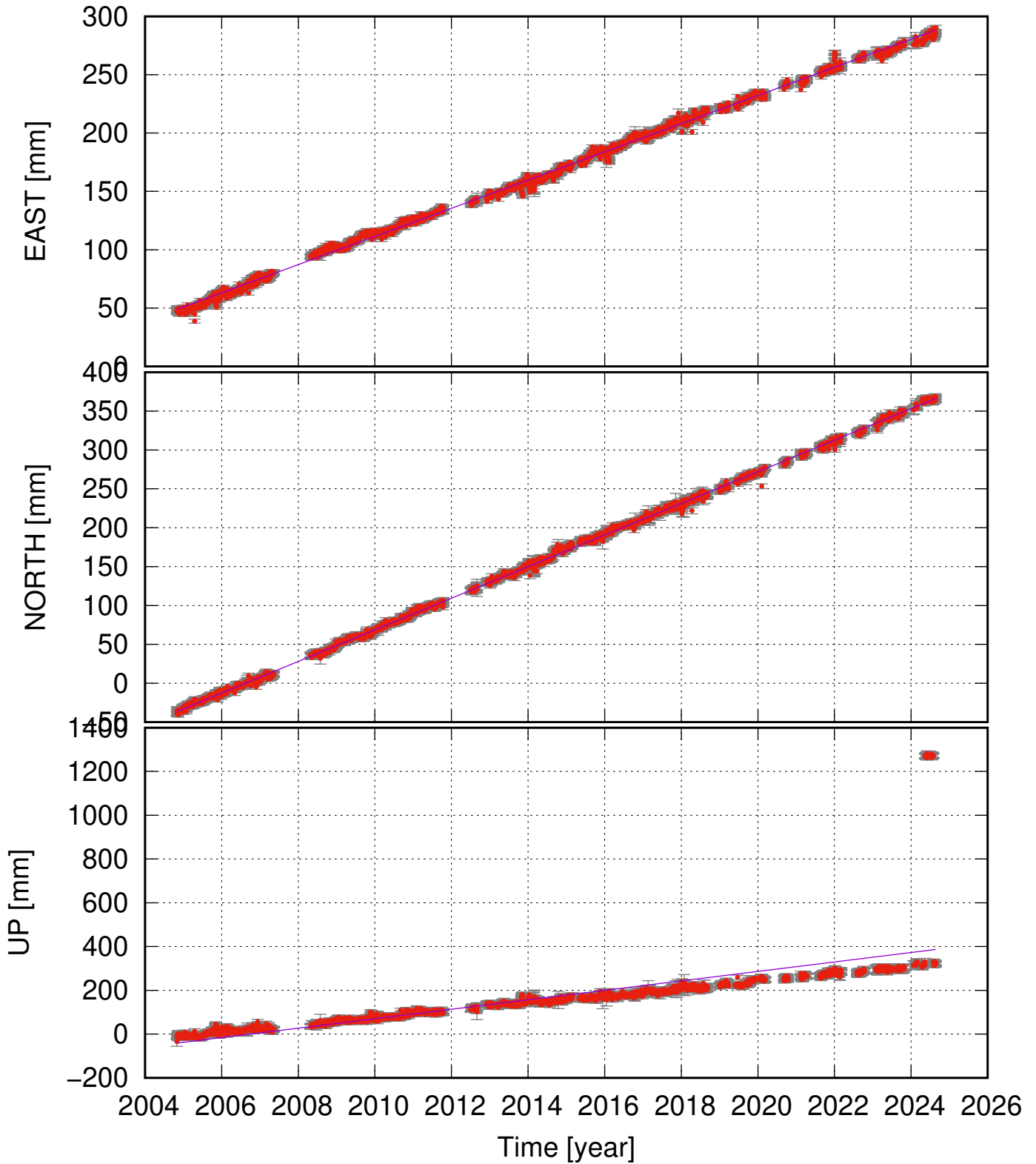
SAUD (64.90, -15.88) time series (ITRF 2014) ve = 12.08 ± 0.14; vn = 20.30 ± 0.12; vu = 21.60 ± 5.76 mm/yr
