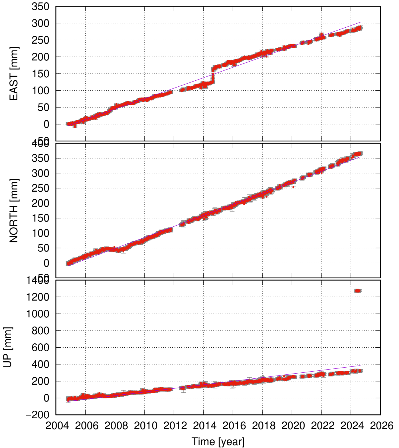
SAUD (64.90, -15.88) time series (ITRF 2014) ve = 15.50 ± 0.54; vn = 18.40 ± 0.37; vu = 21.54 ± 5.57 mm/yr
