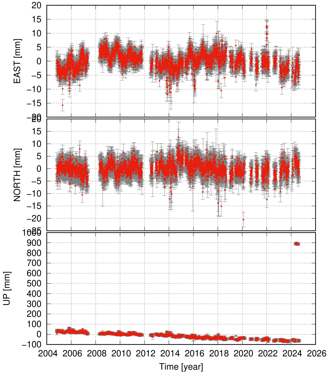
SAUD residual time series (some major events removed as well)
