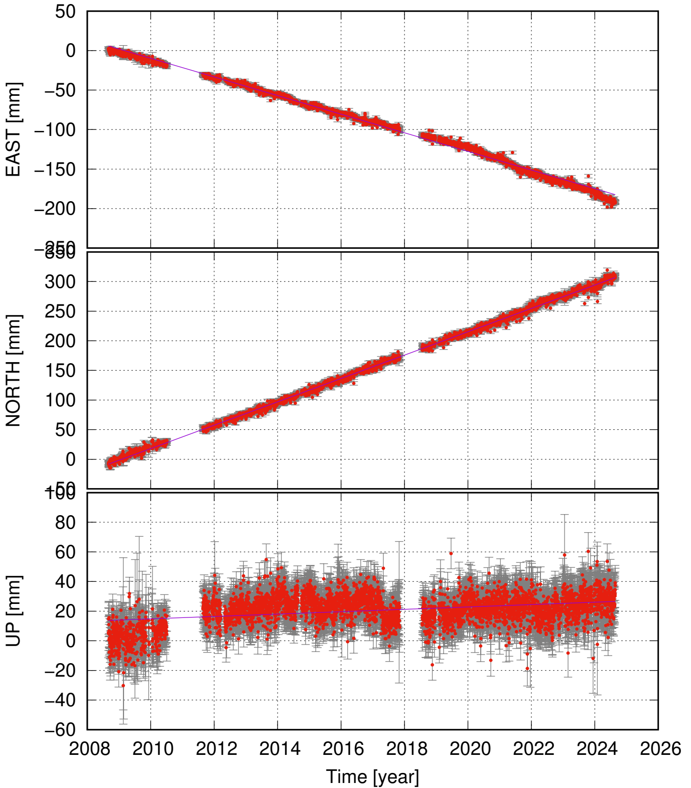
SARP (64.47, -21.27) time series (ITRF 2014) v_e = -11.78 \pm 0.24 ; v_n = 19.72 \pm 0.20 ; v_u = 0.80 \pm 0.57 mm/yr
