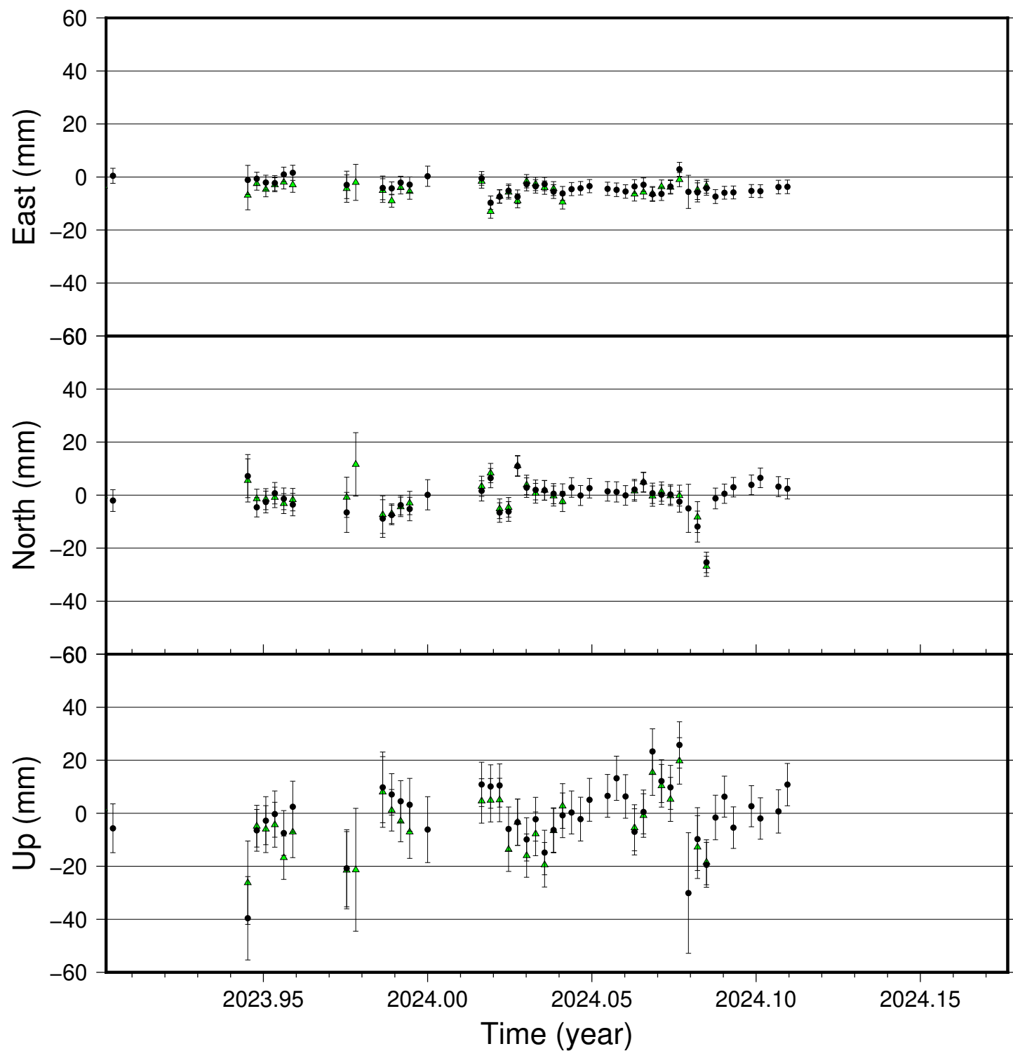
SARP time series (IGS 2014), last 100 days
