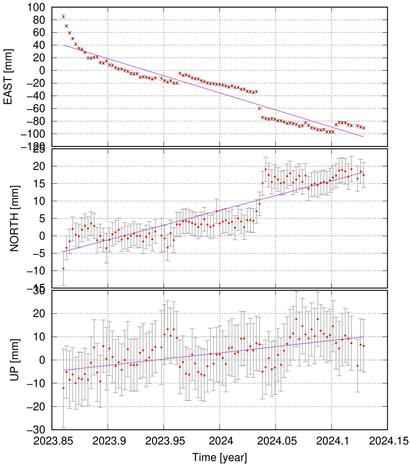
SAFH (63.86, -22.60) time series (ITRF 2014) v_e = -540.31 \pm 49.24 ; v_n = 84.94 \pm 12.53 ; v_u = 53.56 \pm 20.27 mm/yr
