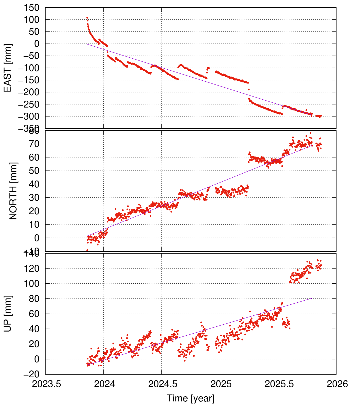
SAFH ( , ) time series (IGb20) ve = +- ; vn = +- ; vu = +- mm/yr
