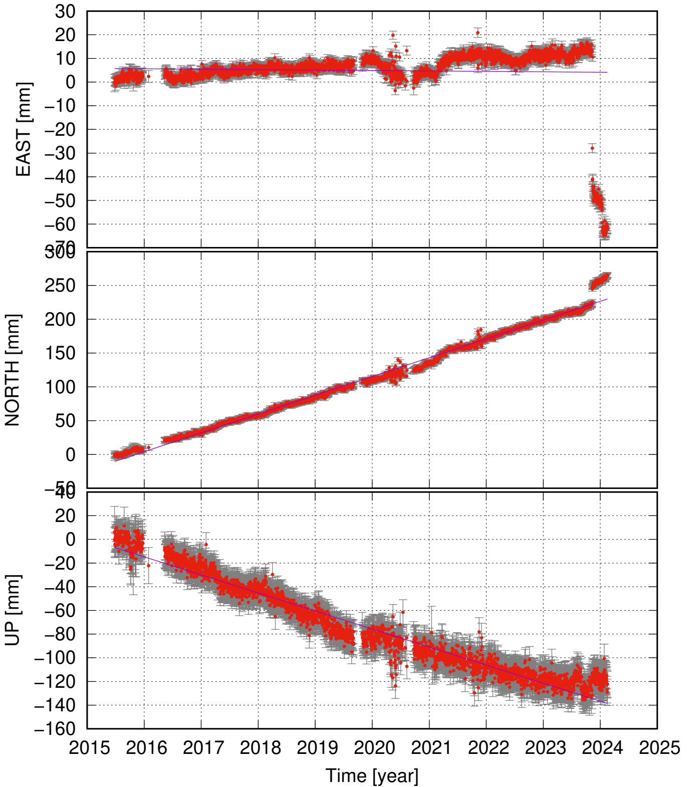
RVIT (63.82, -22.70) time series (ITRF 2014) v_e = -0.18 \pm 1.35 ; v_n = 27.79 \pm 0.83 ; v_u = -15.23 \pm 0.95 mm/yr
