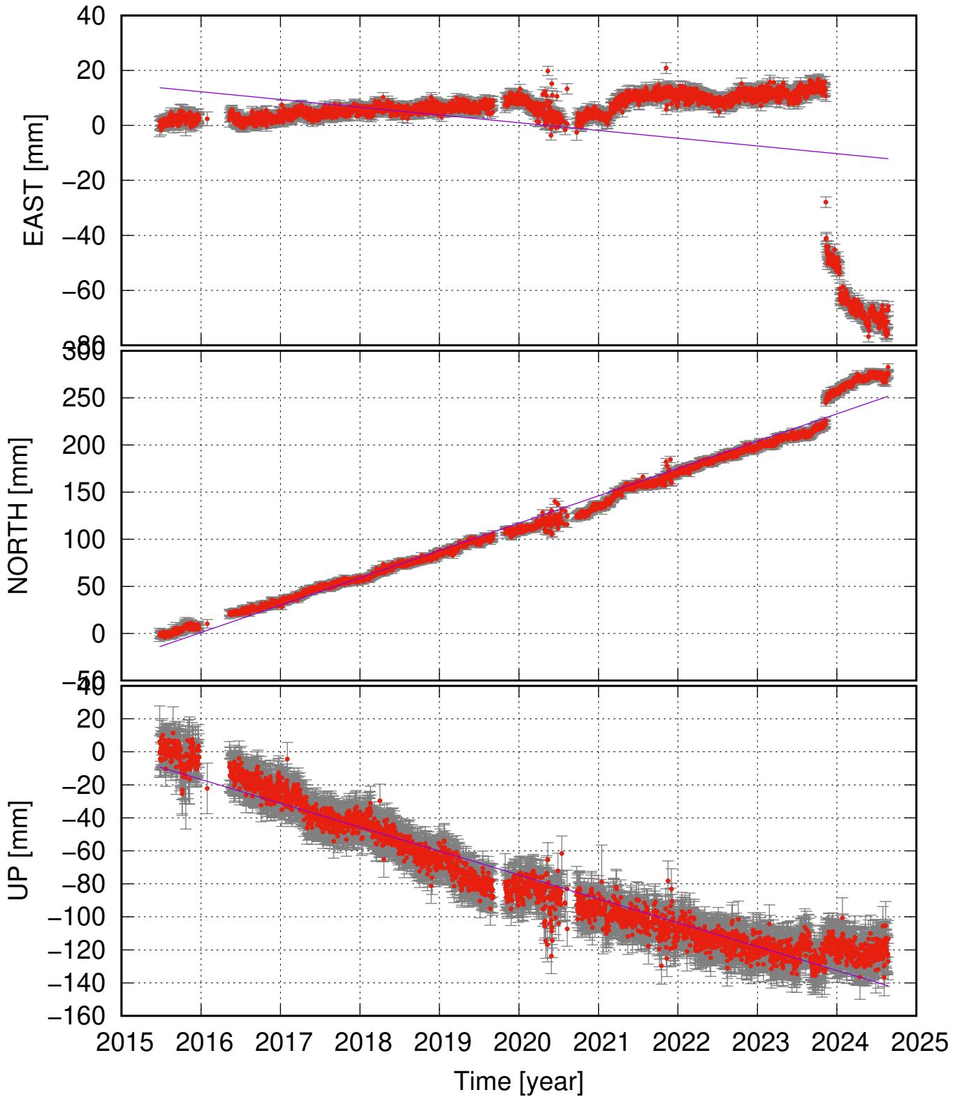
RVIT (63.82, -22.70) time series (ITRF 2014) v_e = -2.81 \pm 2.14 ; v_n = 29.00 \pm 1.12 ; v_u = -14.47 \pm 1.00 mm/yr
