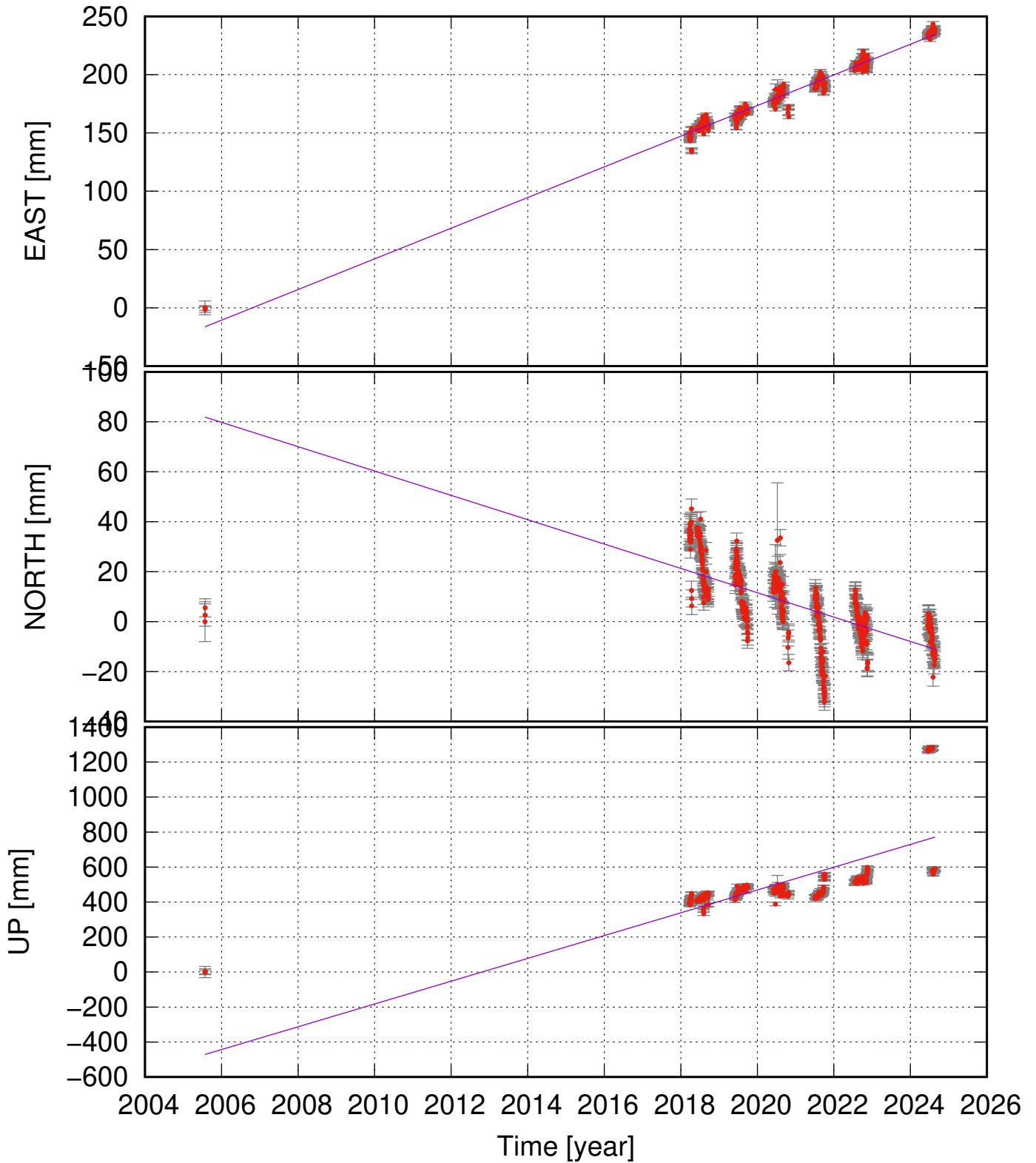
ROTH (63.98, -16.66) time series (ITRF 2014) v_e = 13.15 \pm 0.21 ; v_n = -4.88 \pm 0.62 ; v_u = 65.13 \pm 8.68 mm/yr
