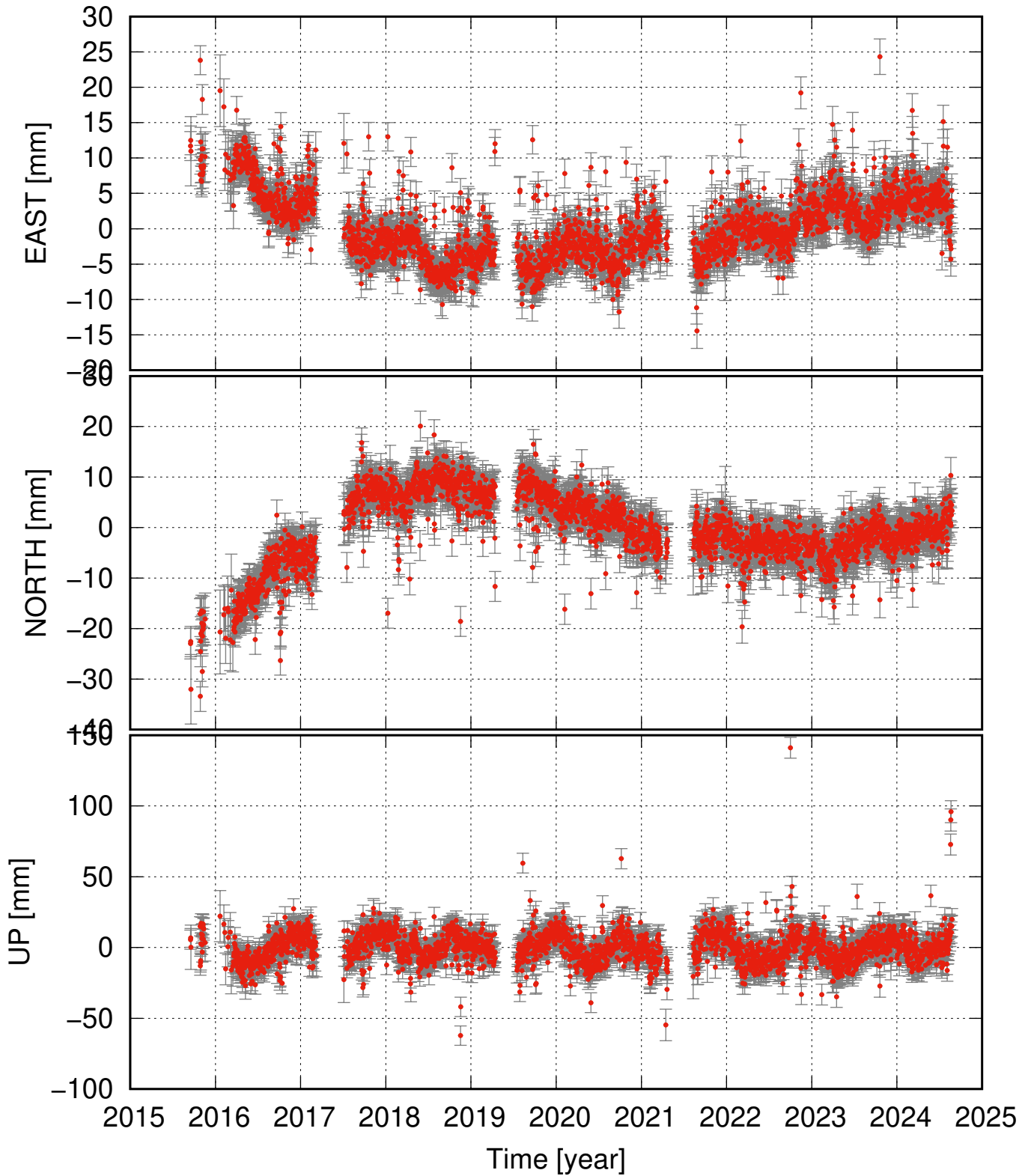
RJUC residual time series (some major events removed as well)
