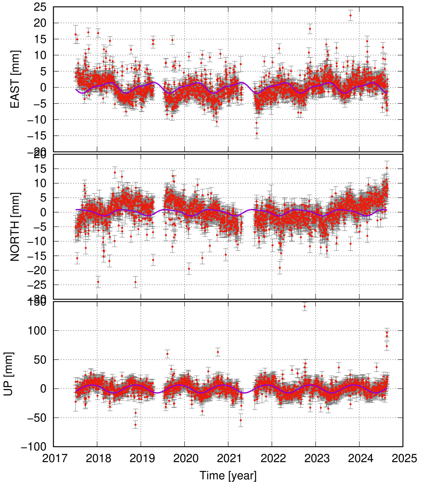
RJUC seasonal fit
