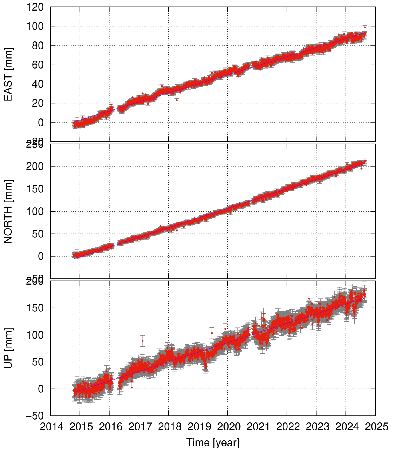
RIFC (64.92, -16.39) time series (ITRF 2014) v_e = 9.41 \pm 0.26 ; v_n = 21.54 \pm 0.31 ; v_u = 17.81 \pm 0.82 mm/yr
