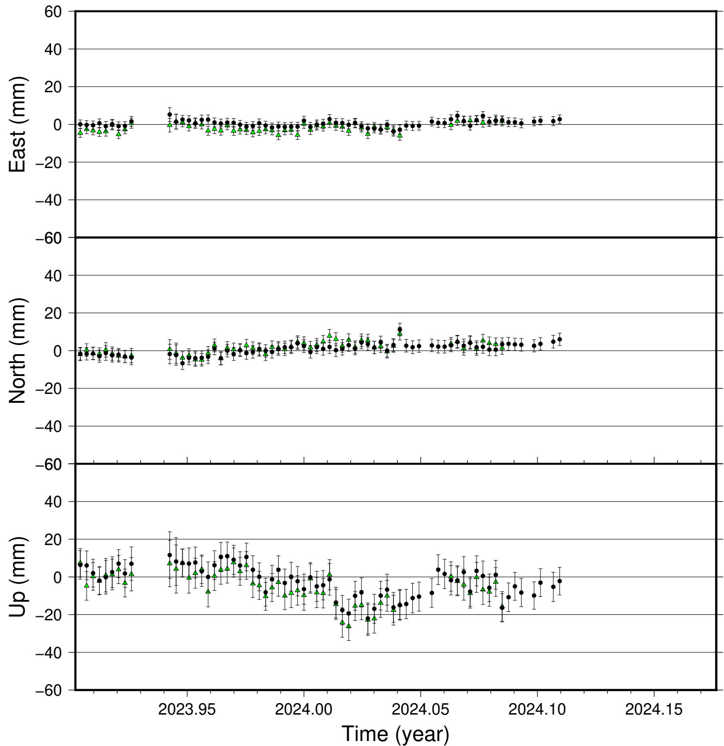
RIFC time series (IGS 2014), last 100 days
