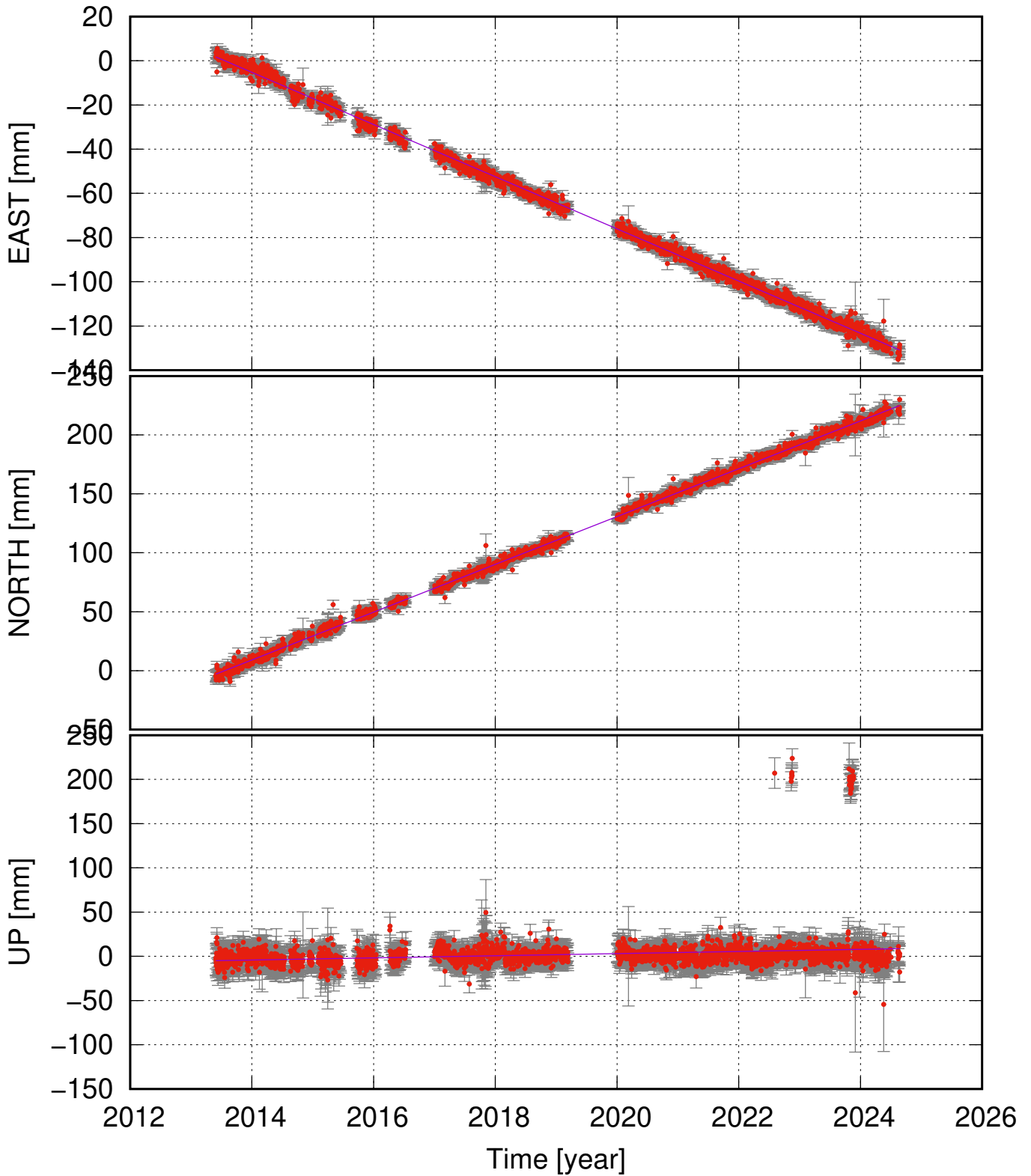
RHOL (65.43, -22.21) time series (ITRF 2014) v_e = -11.81 \pm 0.16 ; v_n = 20.27 \pm 0.21 ; v_u = 1.20 \pm 1.91 mm/yr
