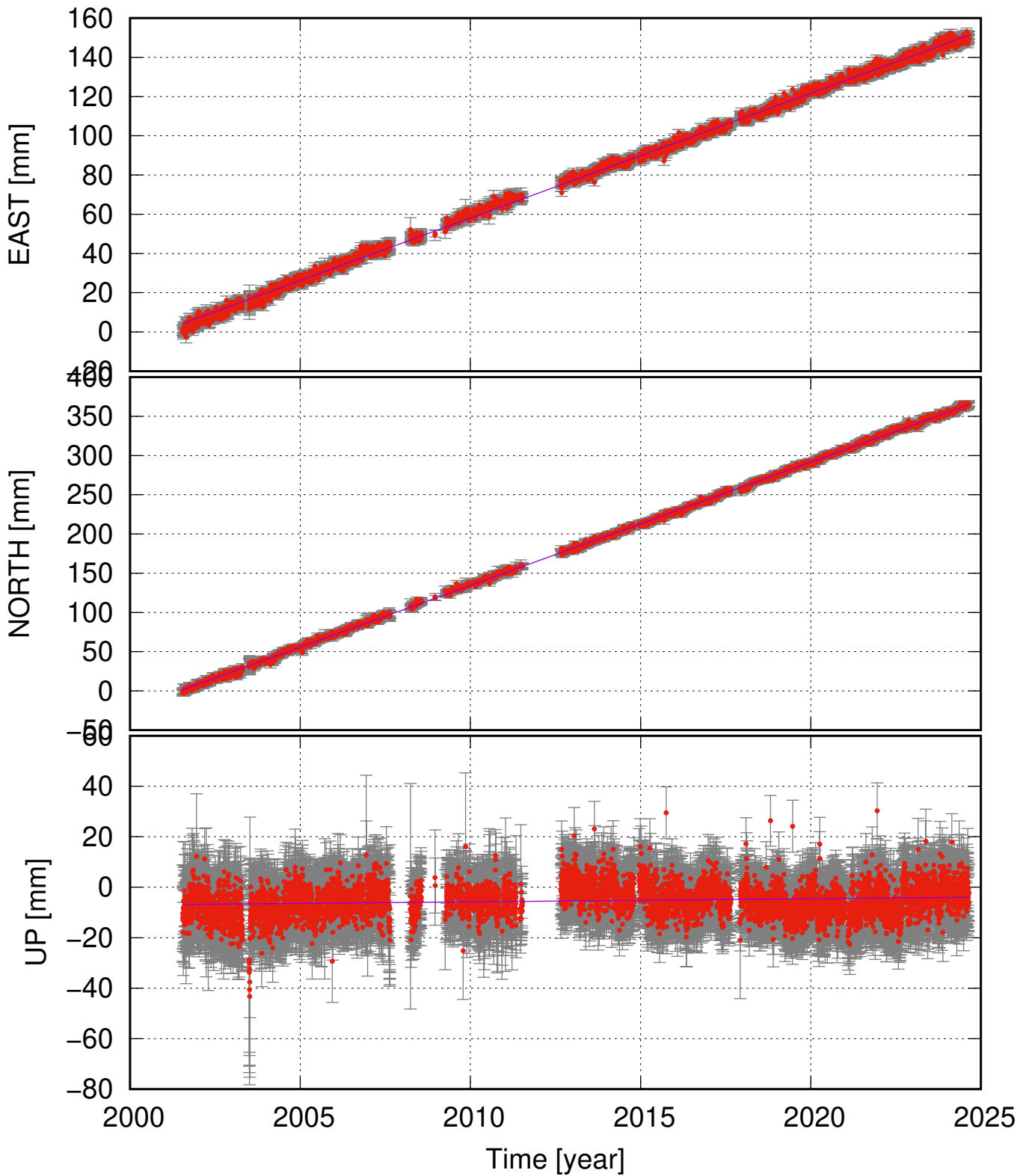
RHOF (66.46, -15.95) time series (ITRF 2014) v_e = 6.36 \pm 0.07 ; v_n = 15.72 \pm 0.08 ; v_u = 0.12 \pm 0.25 mm/yr
