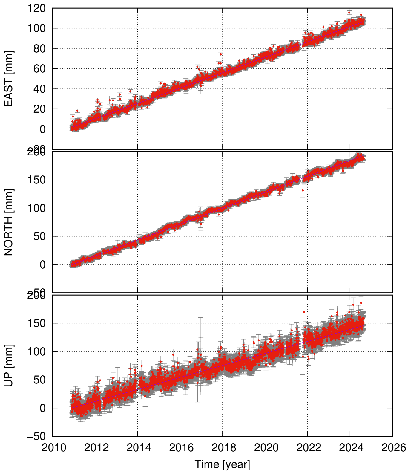
RFEL (63.62, -18.67) time series (ITRF 2014) v_e = 7.62 \pm 0.15 ; v_n = 14.10 \pm 0.22 ; v_u = 10.61 \pm 0.58 mm/yr
