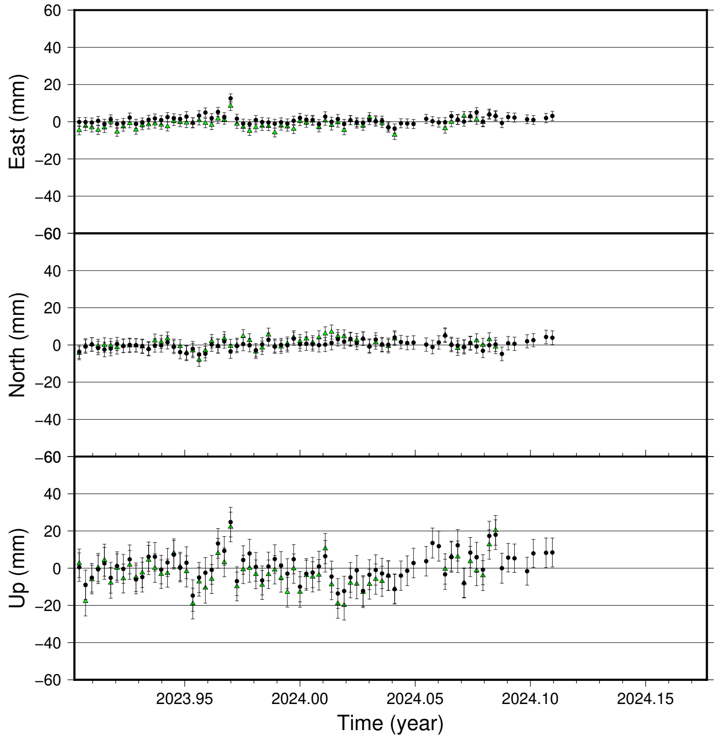
RFEL time series (IGS 2014), last 100 days
