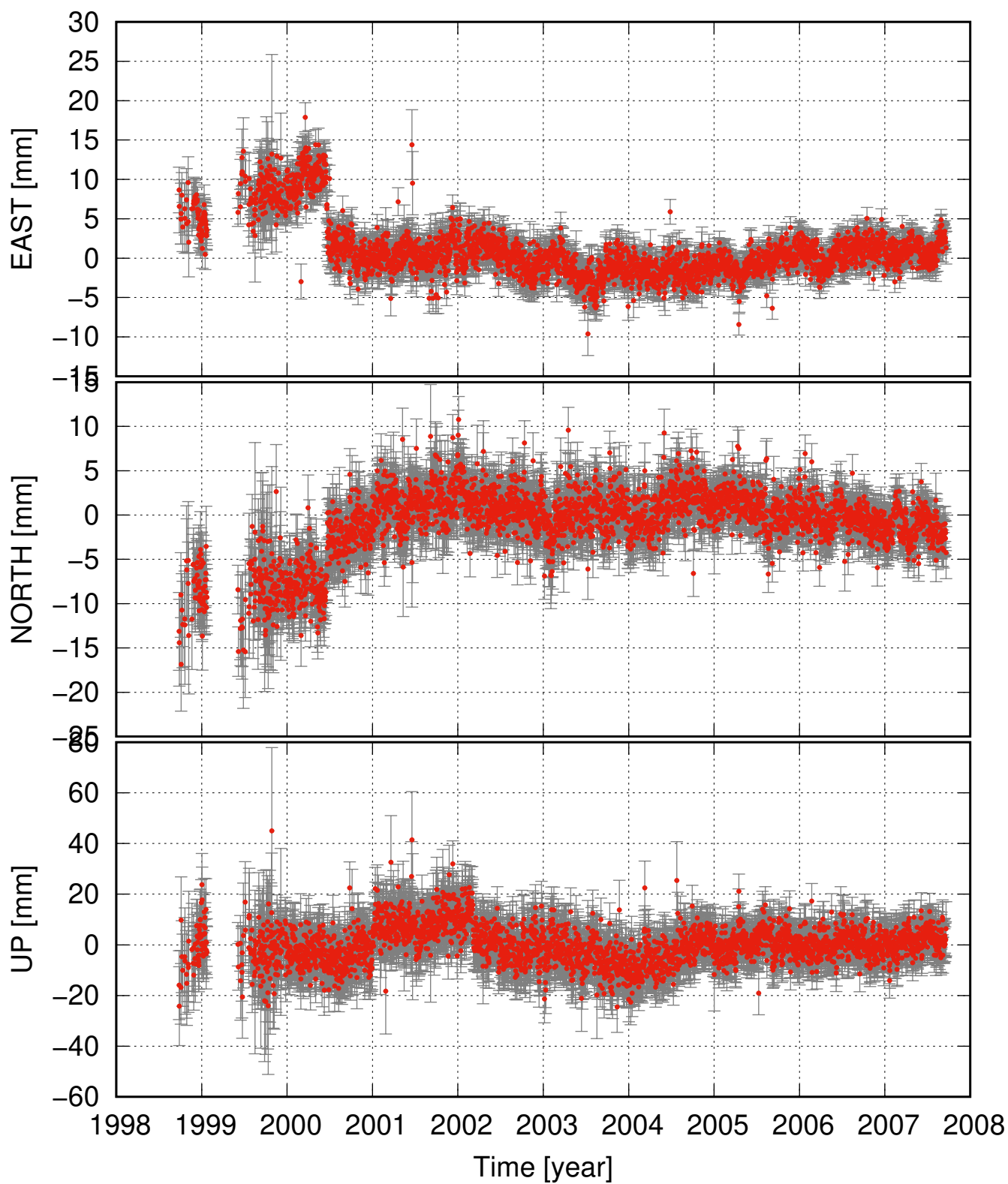
REYZ detrended and seasonal signal removed
