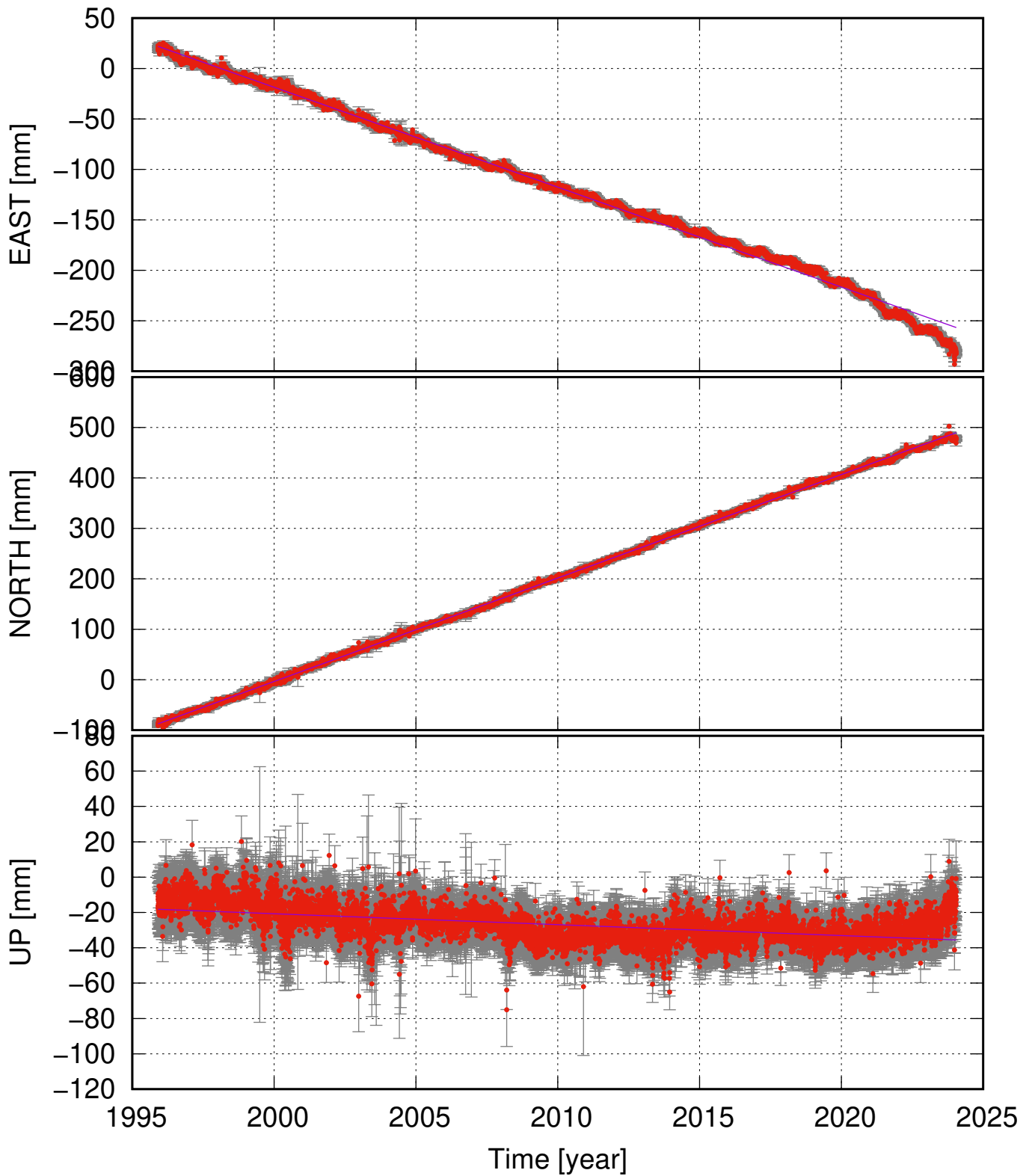
REYK (64.14, -21.96) time series (ITRF 2014) v_e = -9.90 \pm 0.19 ; v_n = 20.51 \pm 0.11 ; v_u = -0.62 \pm 0.27 mm/yr
