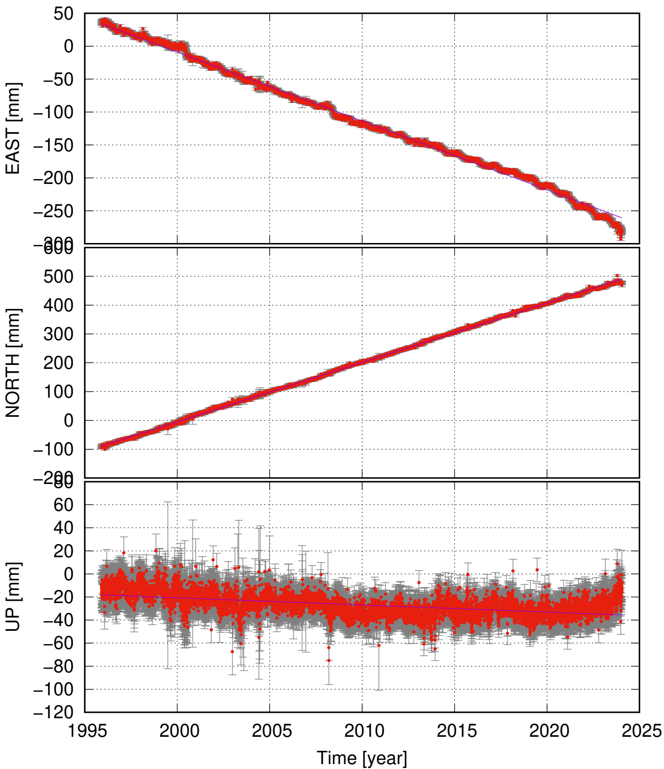
REYK (64.14, -21.96) time series (ITRF 2014) ve = -10.47 \pm 0.19 ; vn = 20.60 \pm 0.13 ; vu = -0.62 \pm 0.27 mm/yr
