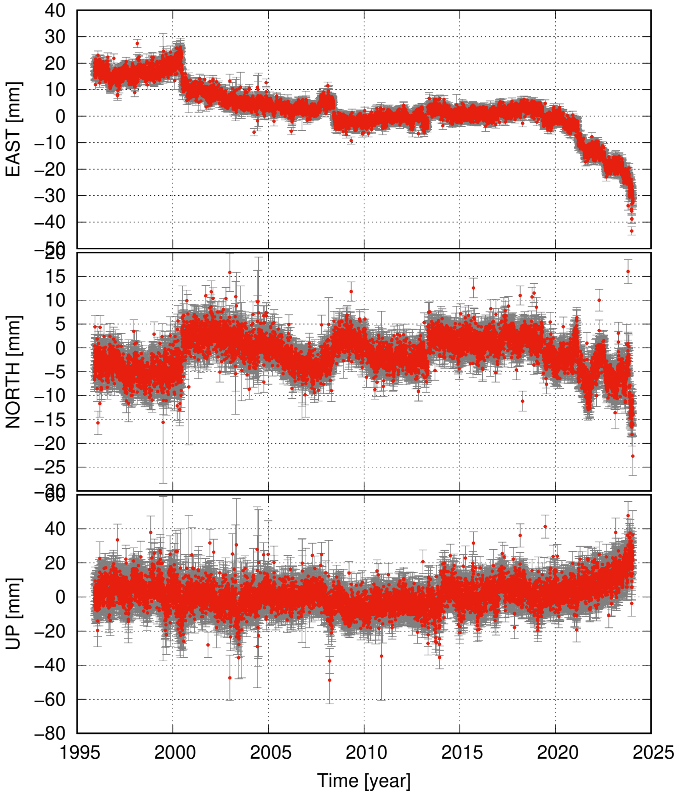
REYK detrended and seasonal signal removed
